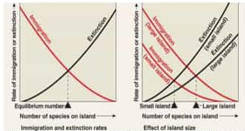
Figure 1. The theory of island biogeography. (a) The interaction of immigration rate and extinction rate produces an equilibrium number of species on an island. (b) In practice, the rate curves bend because some species immigrate more readily than others and because some species are better competitors than others.
