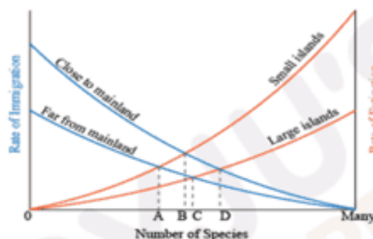
Figure 2. Island biota size varies with distance from the source pool and Island size. An increase in distance, from near far, lowers the immigration rate; an increase in Island areas, from small to large, lowers the extinction rate. The intersection of the immigration and extinction curves yields the equilibrium number of species.
